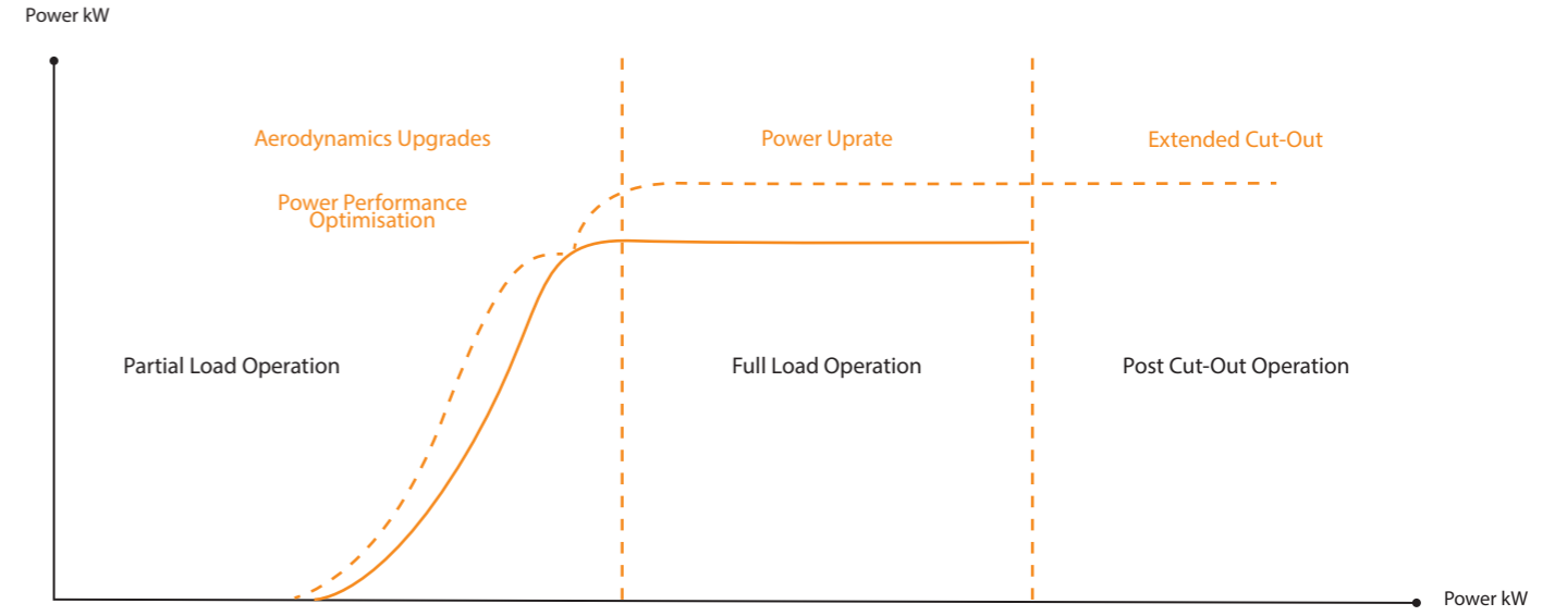
Display of the PowerPlus solutions and their impact on AEP on the different stages of the power curve
