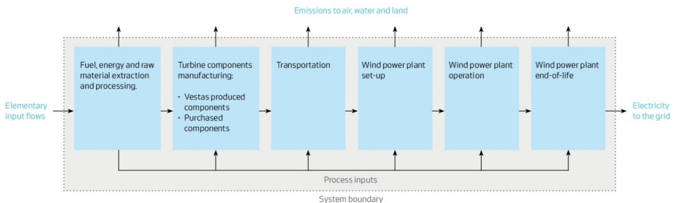
Figure 2: Scope of LCA for a 50MW wind power plant of V90-2.0MW
