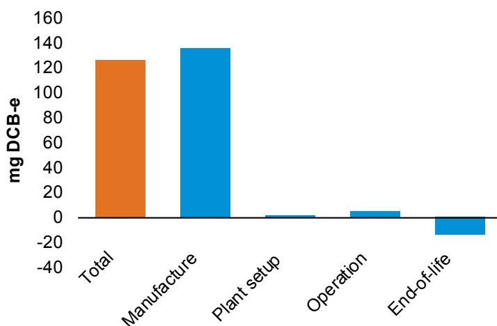
Figure 10: Contribution by life cycle stage to Freshwater aquatic ecotoxicity potential per kWh
