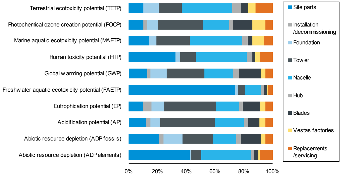
Figure 5: Production and use-phase environmental impacts of V90-2.0MW
