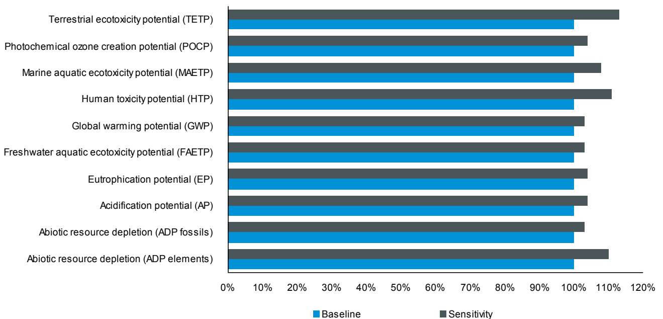
Figure 19: Whole-life sensitivity assessment of doubling replacement parts
