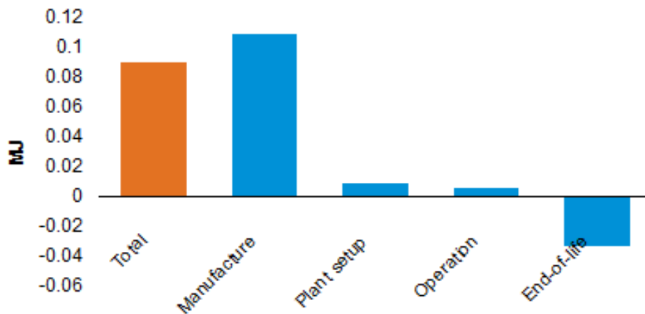
Figure 20: Contribution by life cycle stage to Primary energy from resources (net calorific value) per kWh
