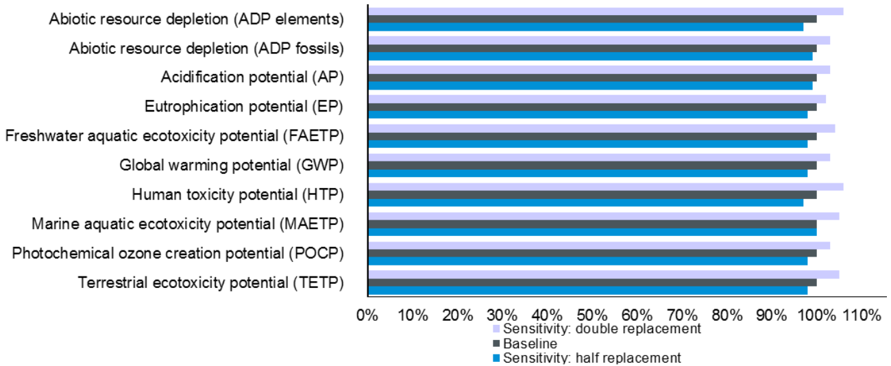
Figure 22: Whole-life sensitivity assessment of doubling or halving replacement parts
