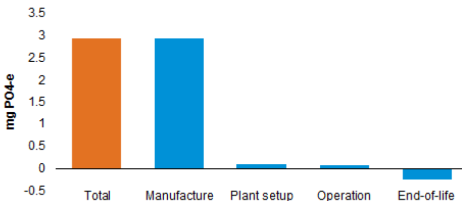
Figure 11: Contribution by life cycle stage to Eutrophication potential per kWh
