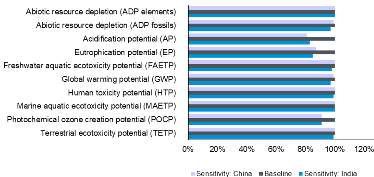
Figure 23: Whole-life sensitivity analysis of transport distances
