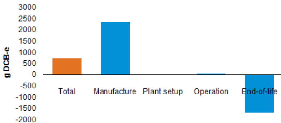
Figure 15: Contribution by life cycle stage to Marine aquatic ecotoxicity potential per kWh
