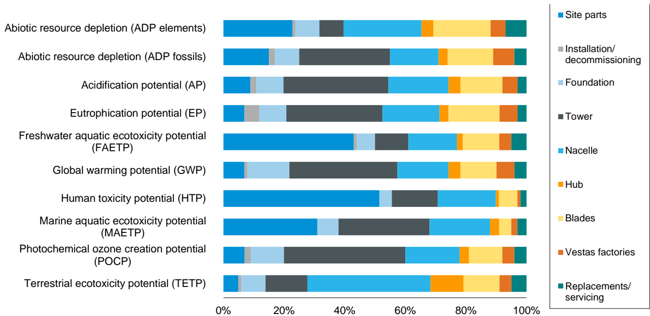
Figure 7: Production and use-phase environmental impacts of V120-2.0 MW
