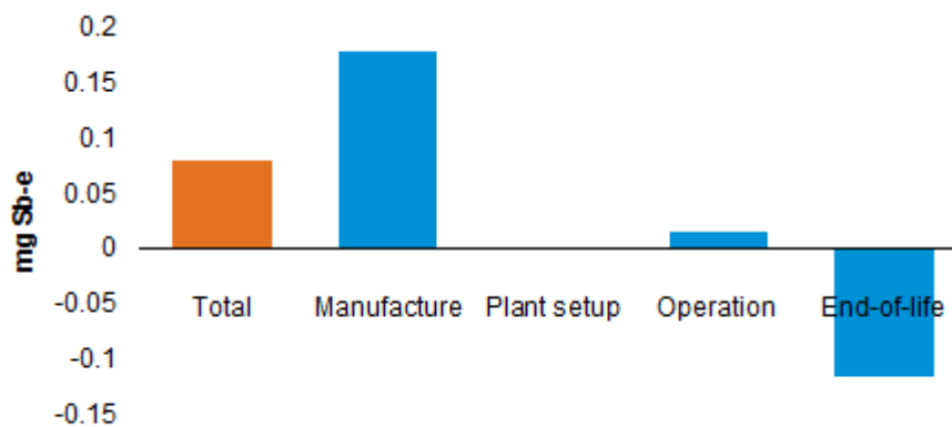
Figure 8: Contribution by life cycle stage to Abiotic resource depletion (element) per kWh
