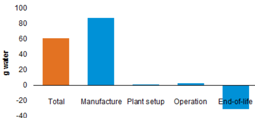
Figure 18: Contribution by life cycle stage to Water consumption per kWh
