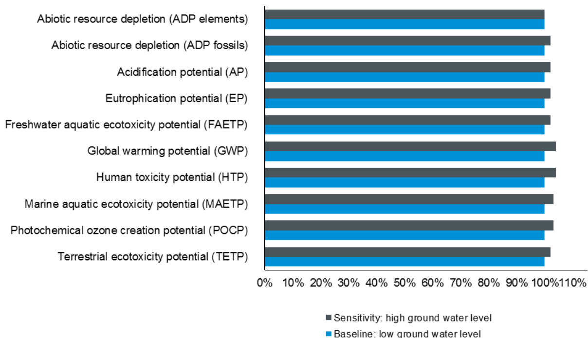
Figure 25: Whole-life impacts for changing from LGWL to a HGWL foundation
