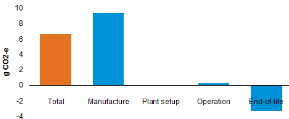
Figure 13: Contribution by life cycle stage to Global warming potential per kWh
