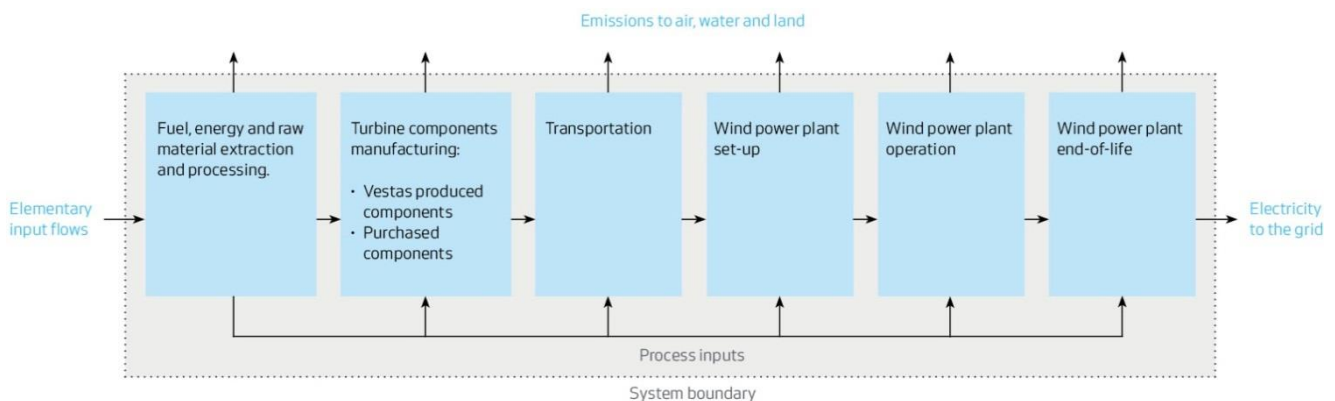
Figure 2: Scope of LCA for a 50MW onshore wind power plant of V120-2.0 MW turbines
