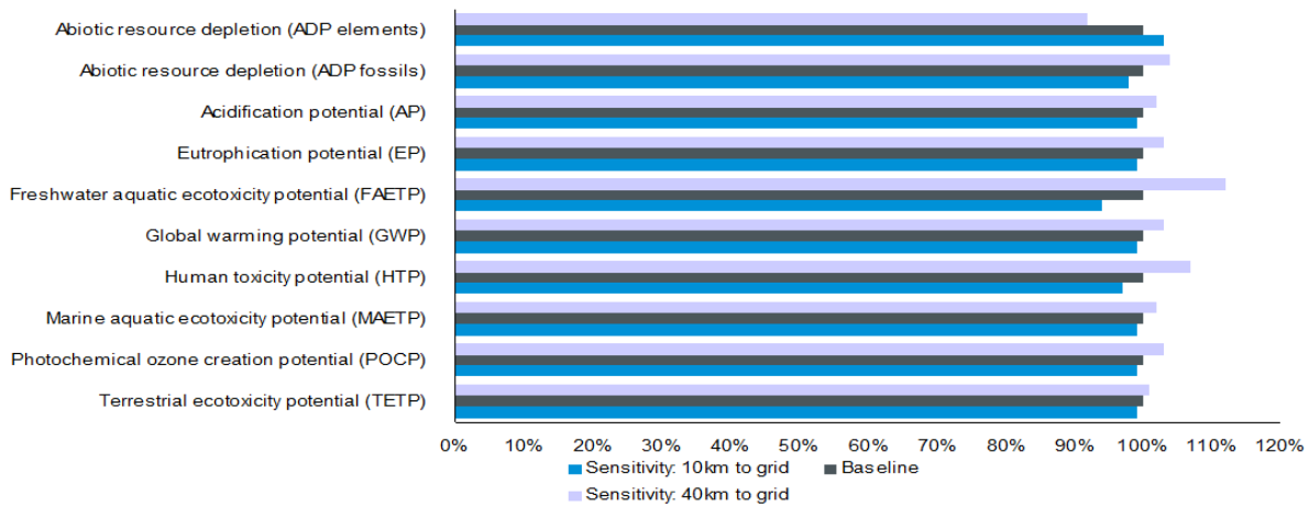
Figure 24: Whole-life impacts for doubling and halving distance to grid to 40km
