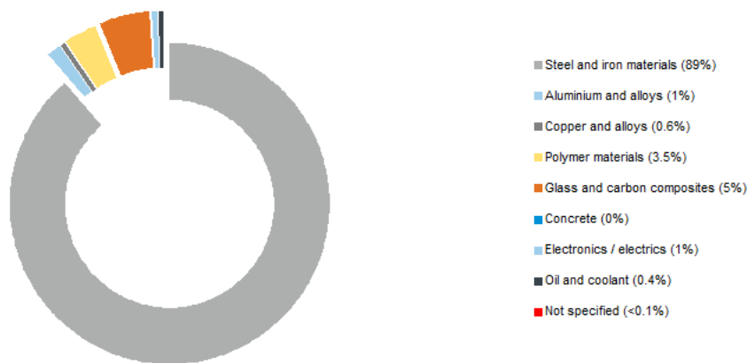
Figure 5: Material breakdown of V126-3.45 MW turbine-only (% mass)
