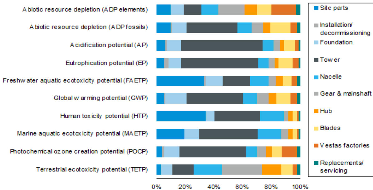
Figure 7: Production and use-phase environmental impacts of V126-3.45 MW
