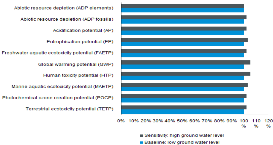
Figure 25: Whole-life impacts for changing from LGWL to a HGWL foundation
