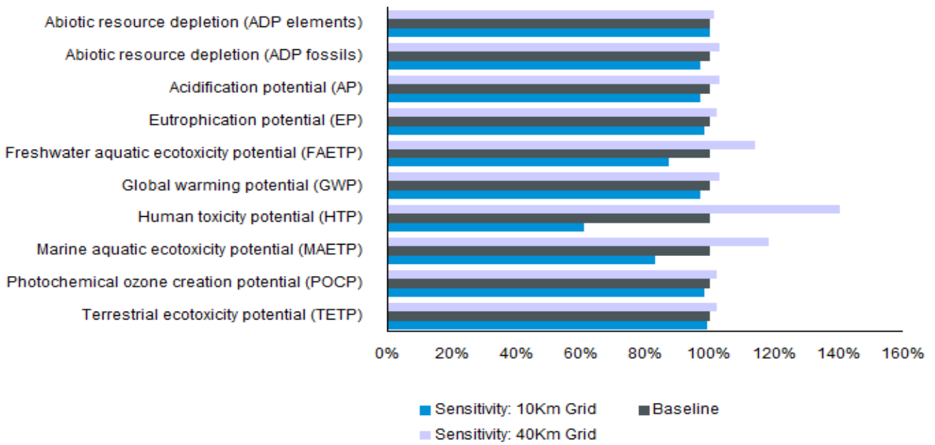
Figure 23: Whole-life impacts for doubling (40km) and halving (10km) distance to grid
