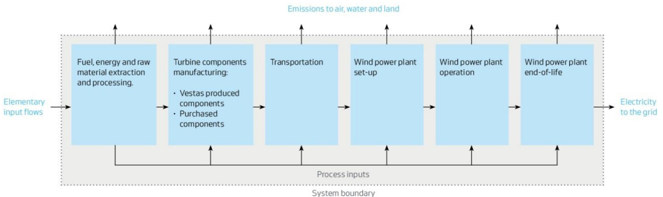
Figure 2: Scope of LCA for a 50MW onshore wind power plant of V100-2.0 MW turbines
