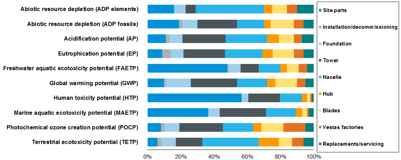
Figure 7: Production and use-phase environmental impacts of V100-2.0 MW
