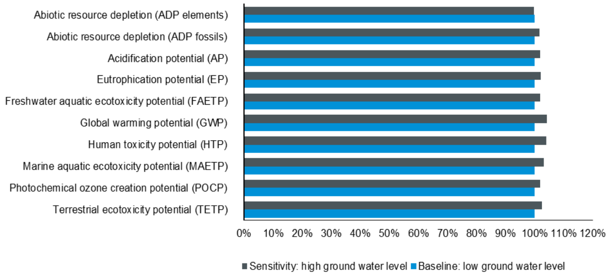
Figure 24: Whole-life impacts for changing from LGWL to a HGWL foundation
