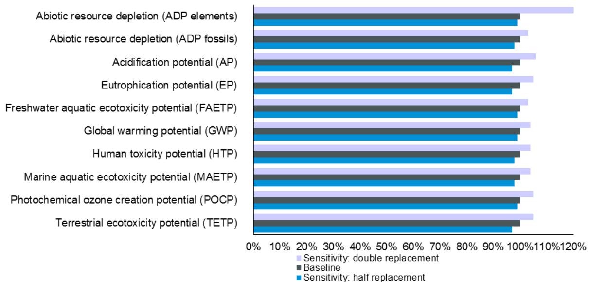
Figure 21: Whole-life sensitivity assessment of doubling or halving replacement parts
