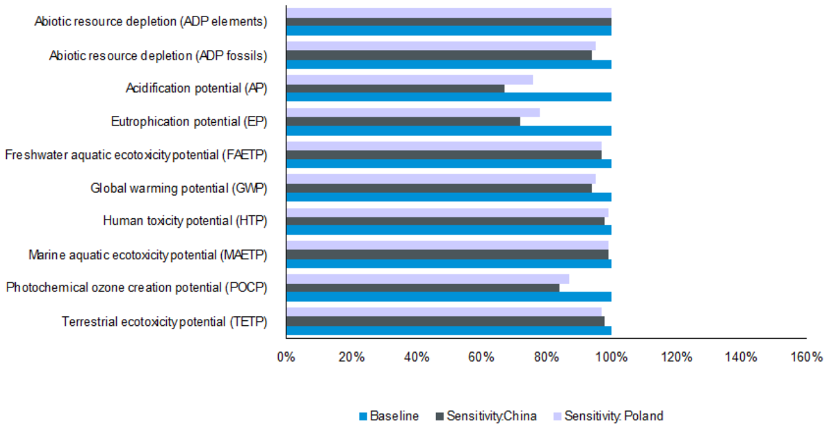
Figure 22: Whole-life sensitivity analysis of transport distances
