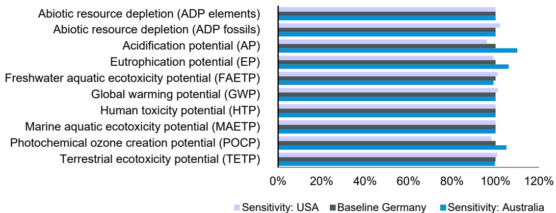
Figure 23: Whole-life sensitivity analysis of transport distances
