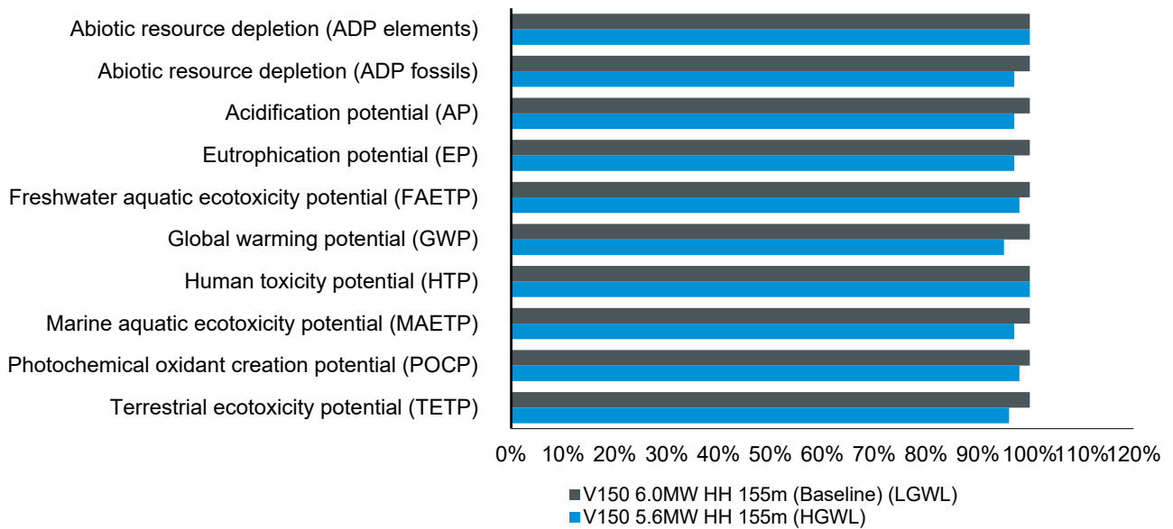
Figure 25: Whole-life impacts for changing from LGWL to a HGWL foundation
