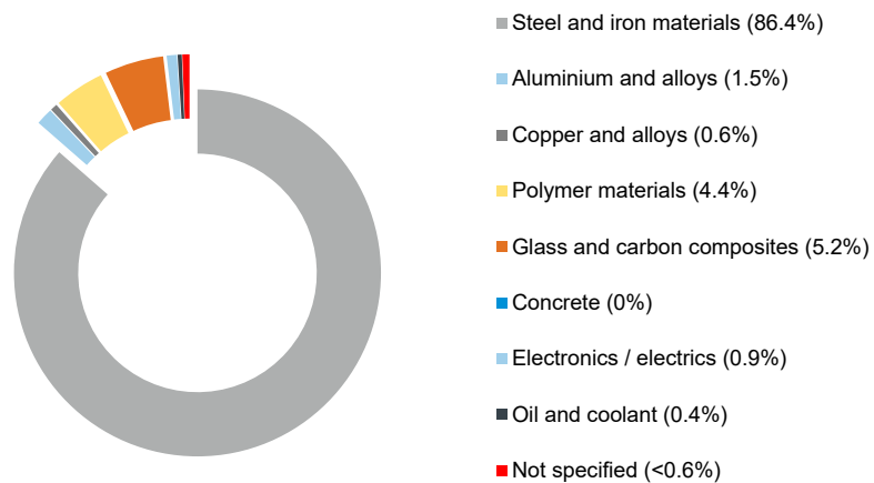
Figure 6: Material breakdown of 100MW power plant of V150-6.0 MW turbines (% mass)
