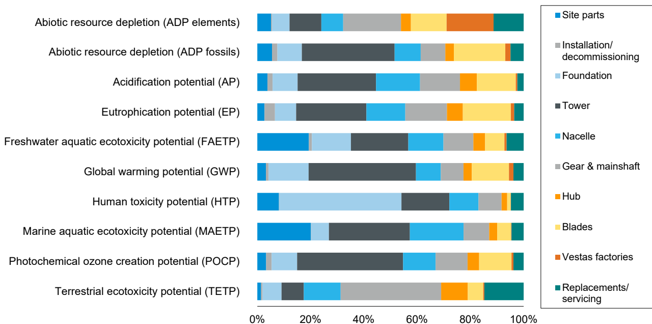
Figure 7: Production and use-phase environmental impacts of V150-6.0 MW
