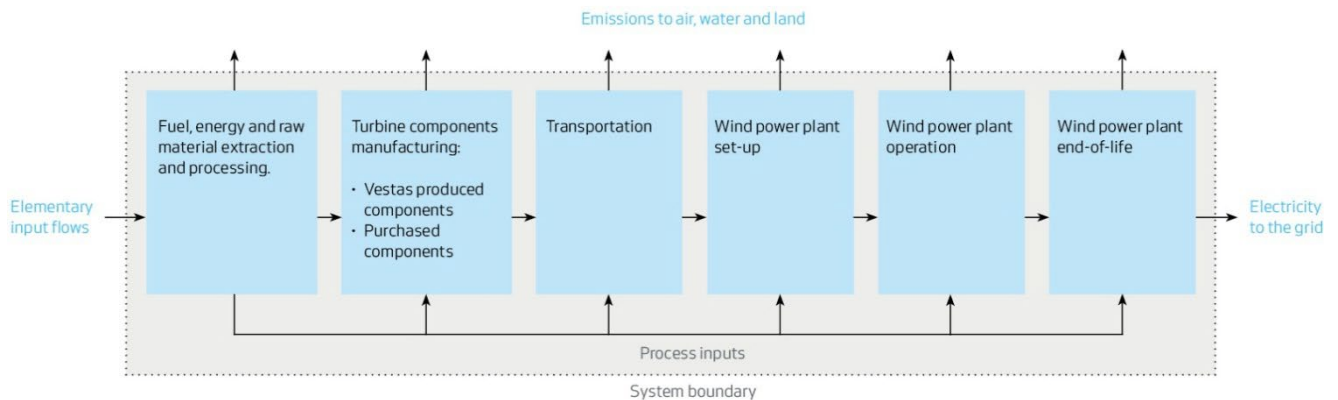
Figure 2: Scope of LCA for a 100MW onshore wind power plant of EnVentus V150-6.0 MW turbines
